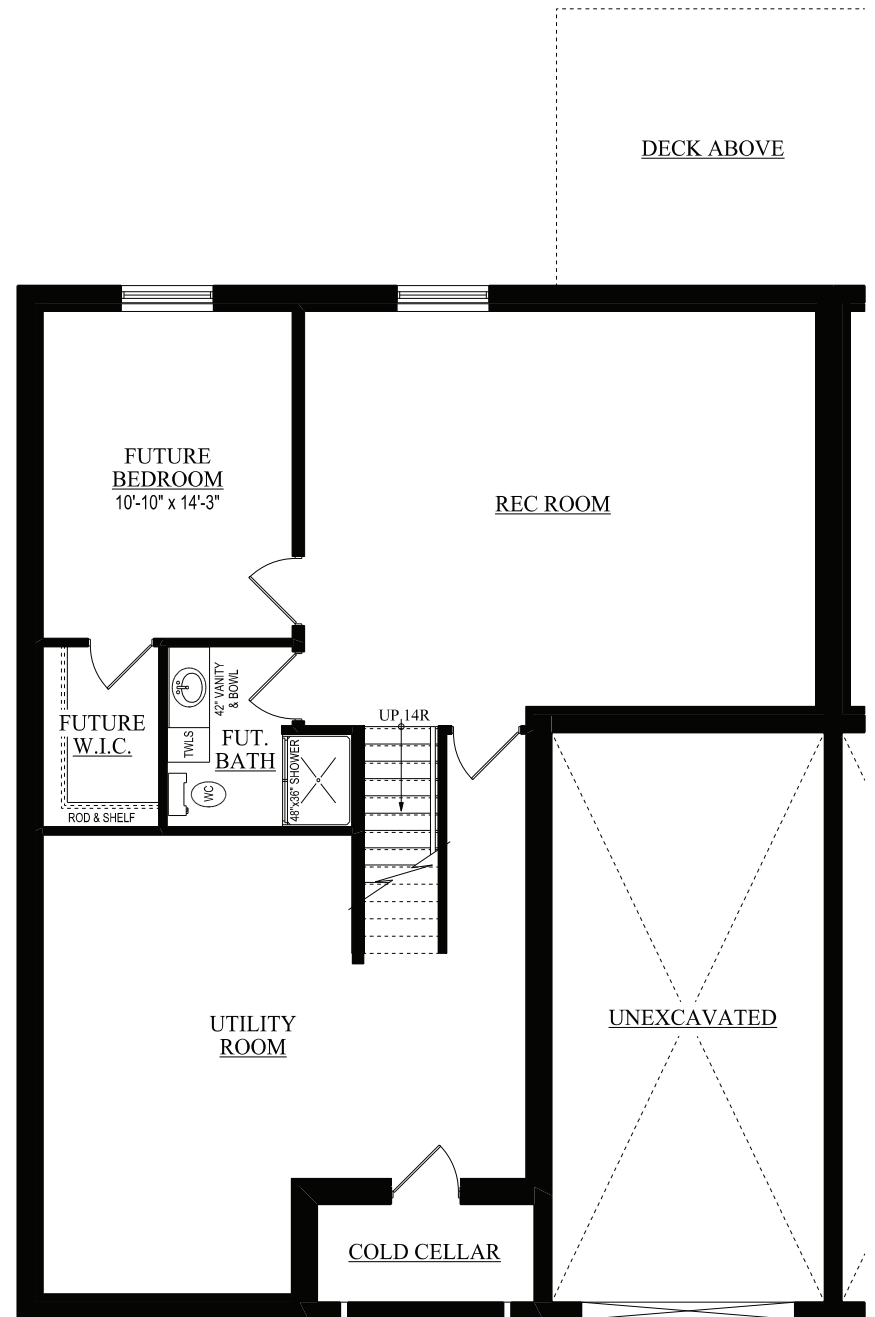
Unit Foundation Plan
