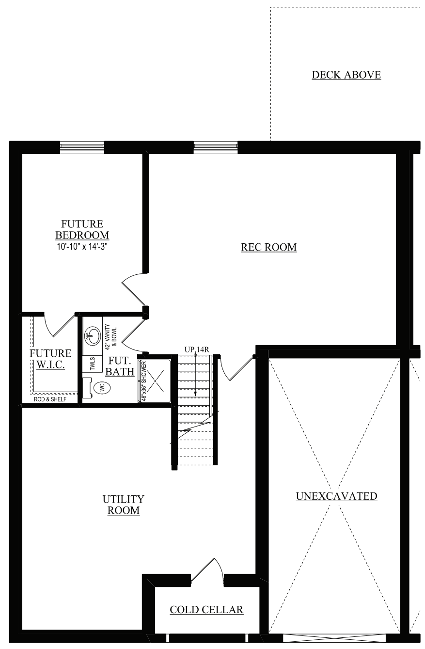
Unit Foundation Plan
